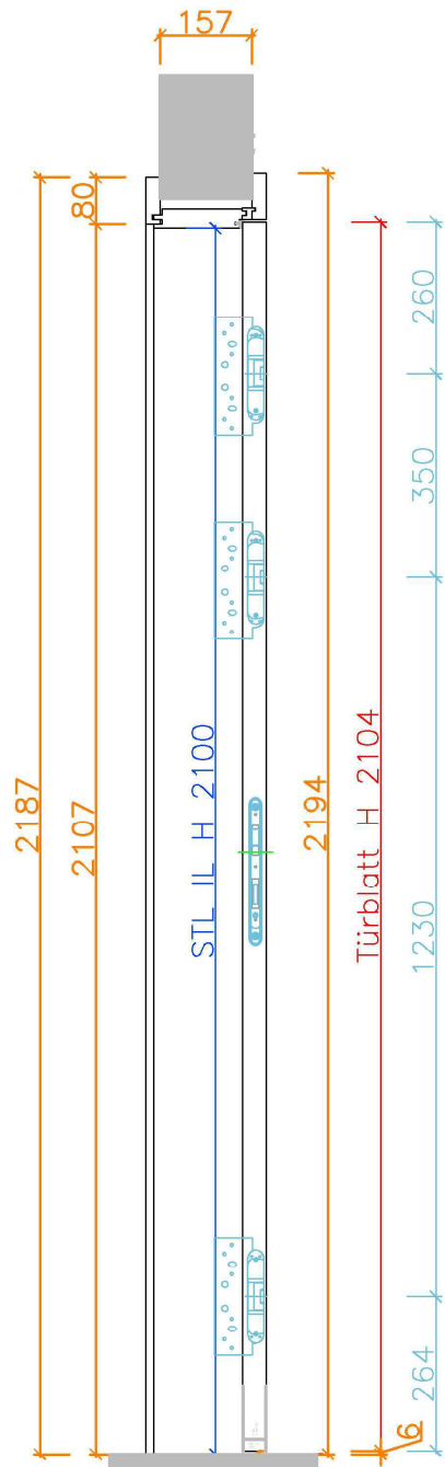
Detail D
